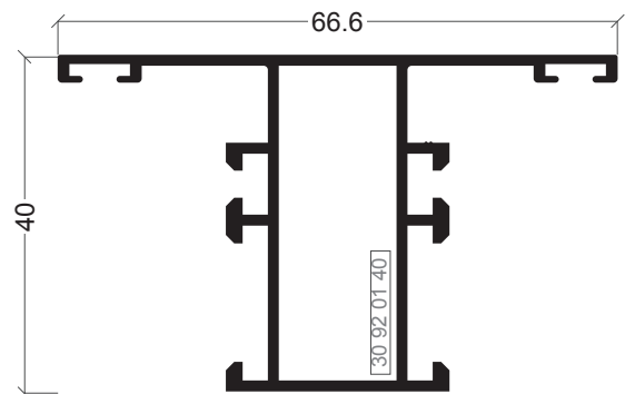
AZ-01 Travessa
