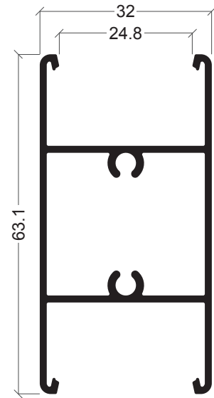
XP-25 Travessa 63 mm
