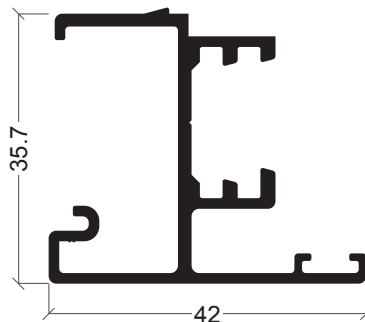
BE-04 Inversor
